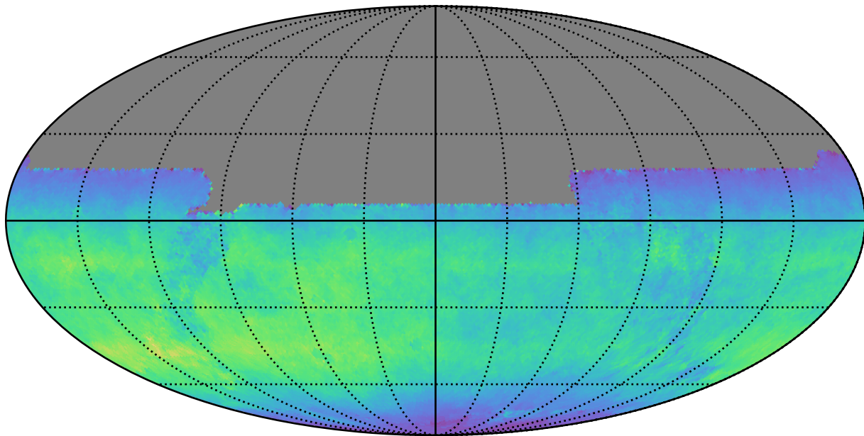
too_elab_r64_d2_giz_v3.4_10yrs All sky y band: Normalized Teff
