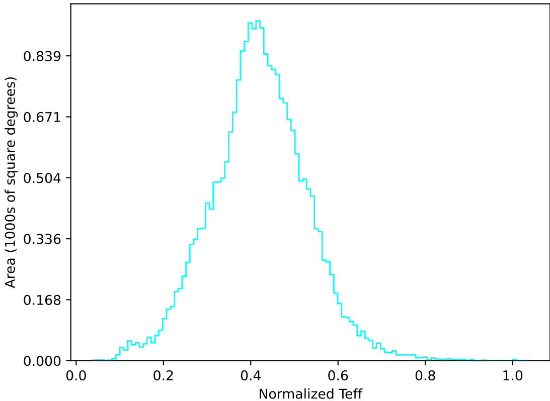
too_elab_r64_d2_giz_v3.4_10yrs All sky u band: Normalized Teff
