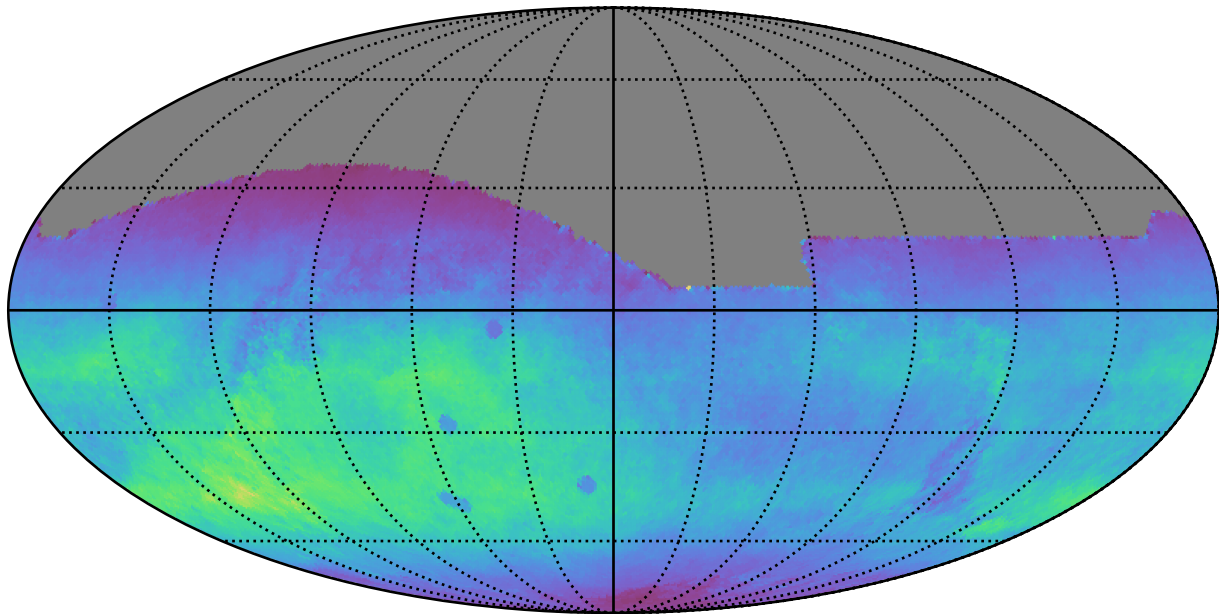
too_elab_r64_d2_giz_v3.4_10yrs All sky r band: Normalized Teff
