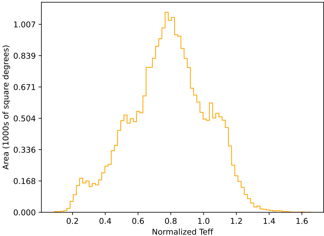
too_elab_r64_d2_giz_v3.4_10yrs All sky r band: Normalized Teff
