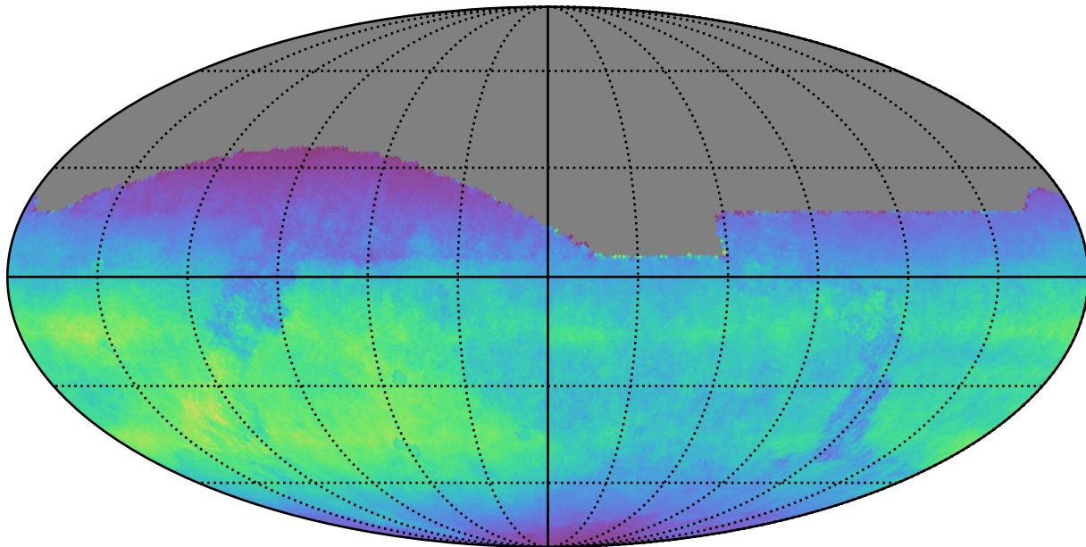
too_elab_r64_d2_giz_v3.4_10yrs All sky i band: Normalized Teff
