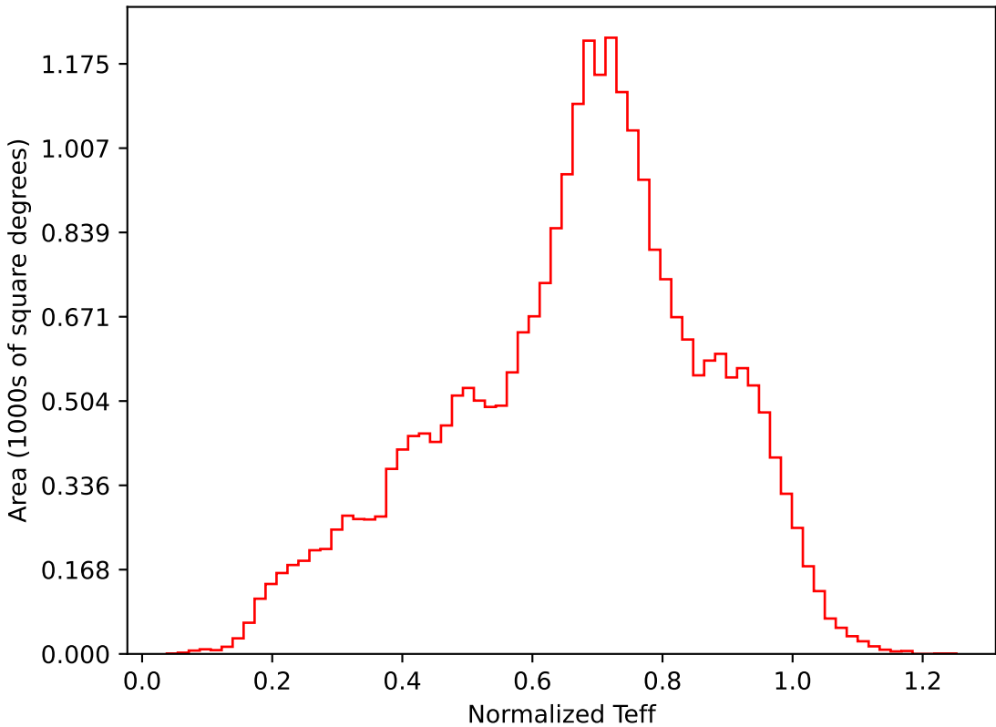
too_elab_r64_d2_giz_v3.4_10yrs All sky i band: Normalized Teff
