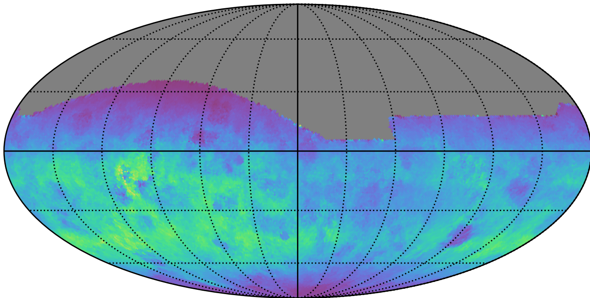
too_elab_r64_d2_giz_v3.4_10yrs All sky g band: Normalized Teff
