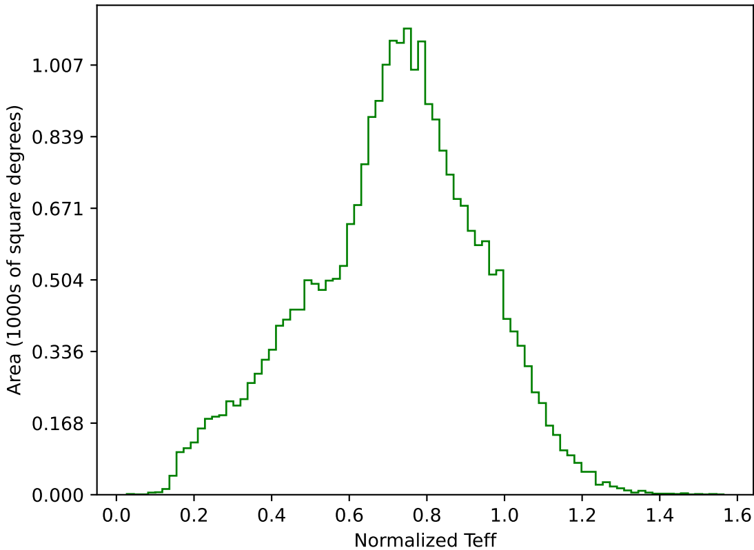
too_elab_r64_d2_giz_v3.4_10yrs All sky g band: Normalized Teff
