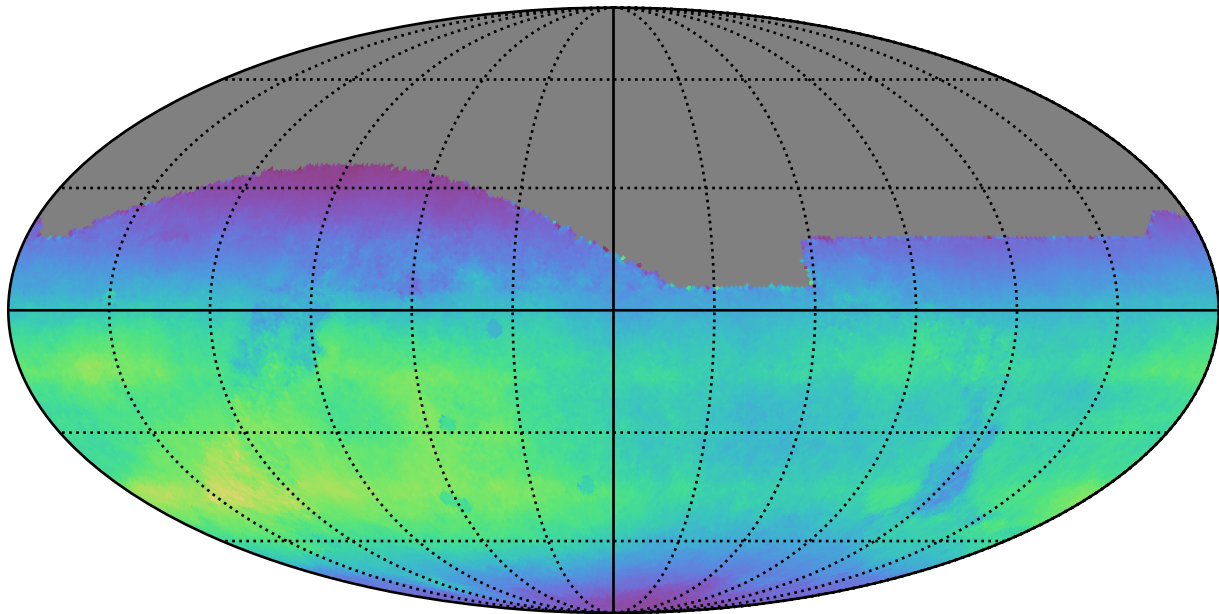
too_elab_r64_d2_giz_v3.4_10yrs All sky all bands: Normalized Teff
