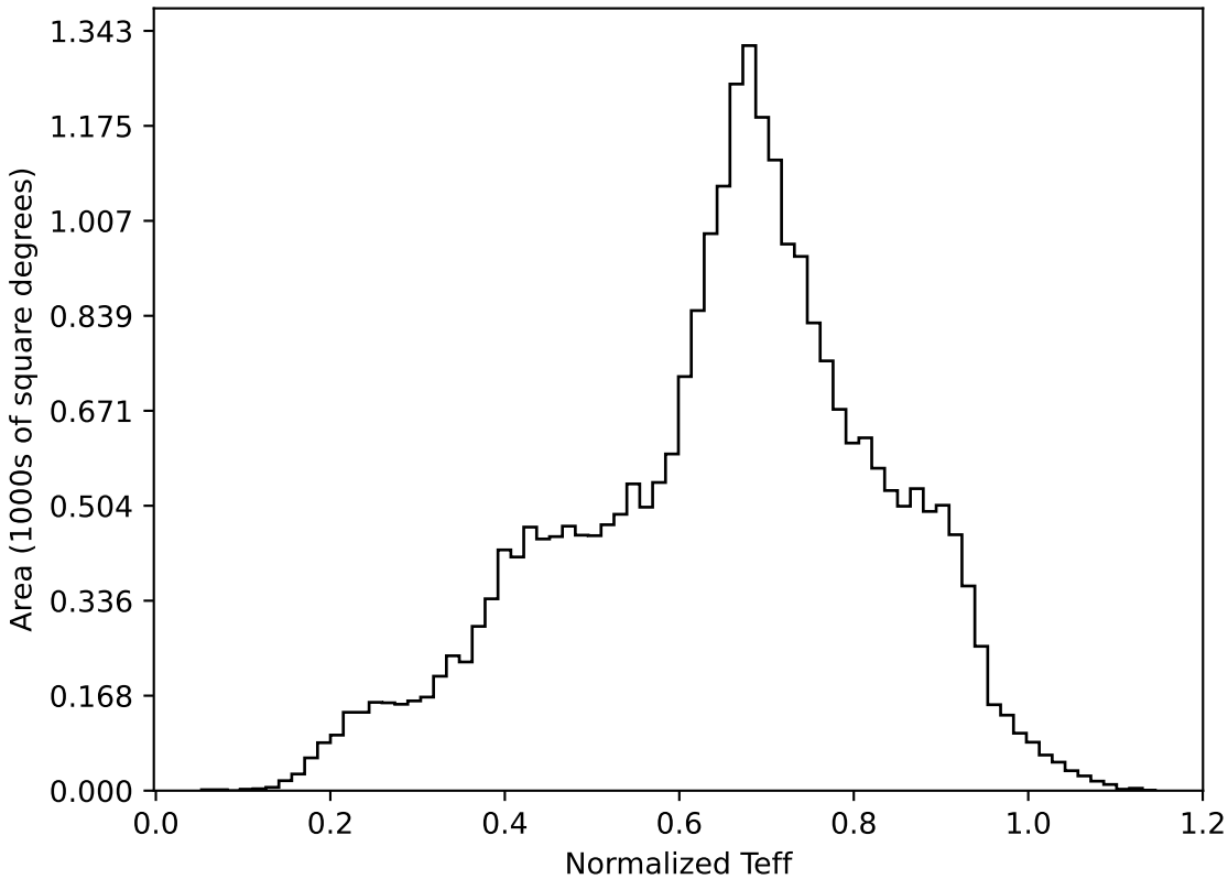
too_elab_r64_d2_giz_v3.4_10yrs All sky all bands: Normalized Teff
