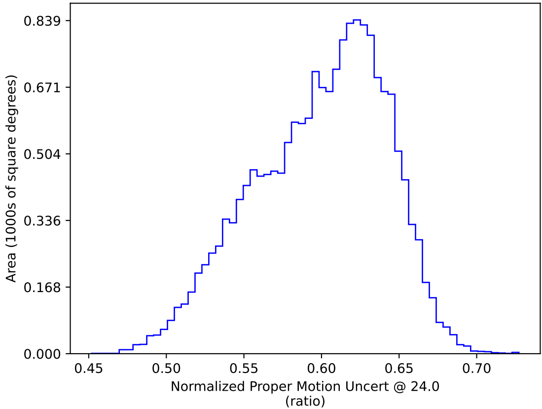
too_elab_r64_d2_giz_v3.4_10yrs WFD: Normalized Proper Motion Uncert @ 24.0
