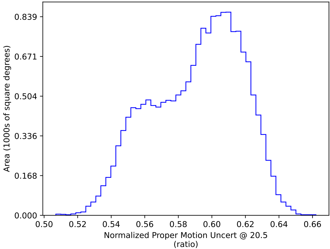
too_elab_r64_d2_giz_v3.4_10yrs WFD: Normalized Proper Motion Uncert @ 20.5
