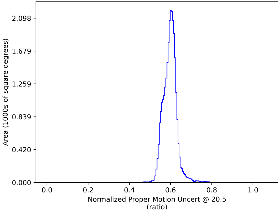
too_elab_r64_d2_giz_v3.4_10yrs All sky: Normalized Proper Motion Uncert @ 20.5
