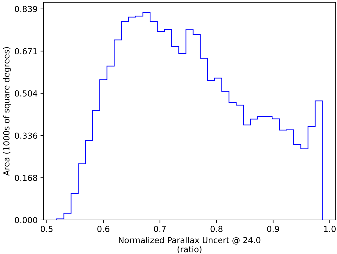
too_elab_r64_d2_giz_v3.4_10yrs WFD: Normalized Parallax Uncert @ 24.0
