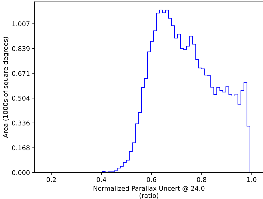
too_elab_r64_d2_giz_v3.4_10yrs All sky: Normalized Parallax Uncert @ 24.0
