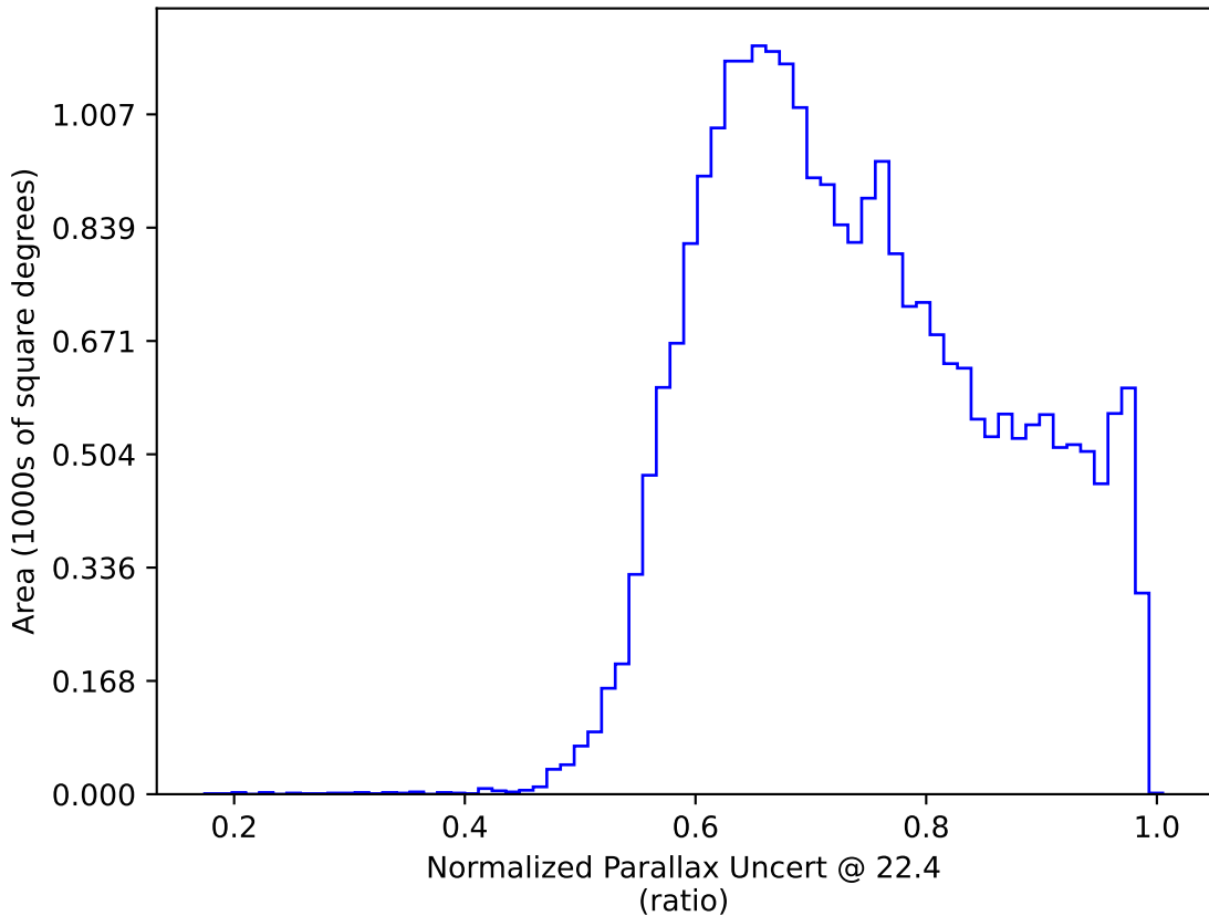
too_elab_r64_d2_giz_v3.4_10yrs All sky: Normalized Parallax Uncert @ 22.4
