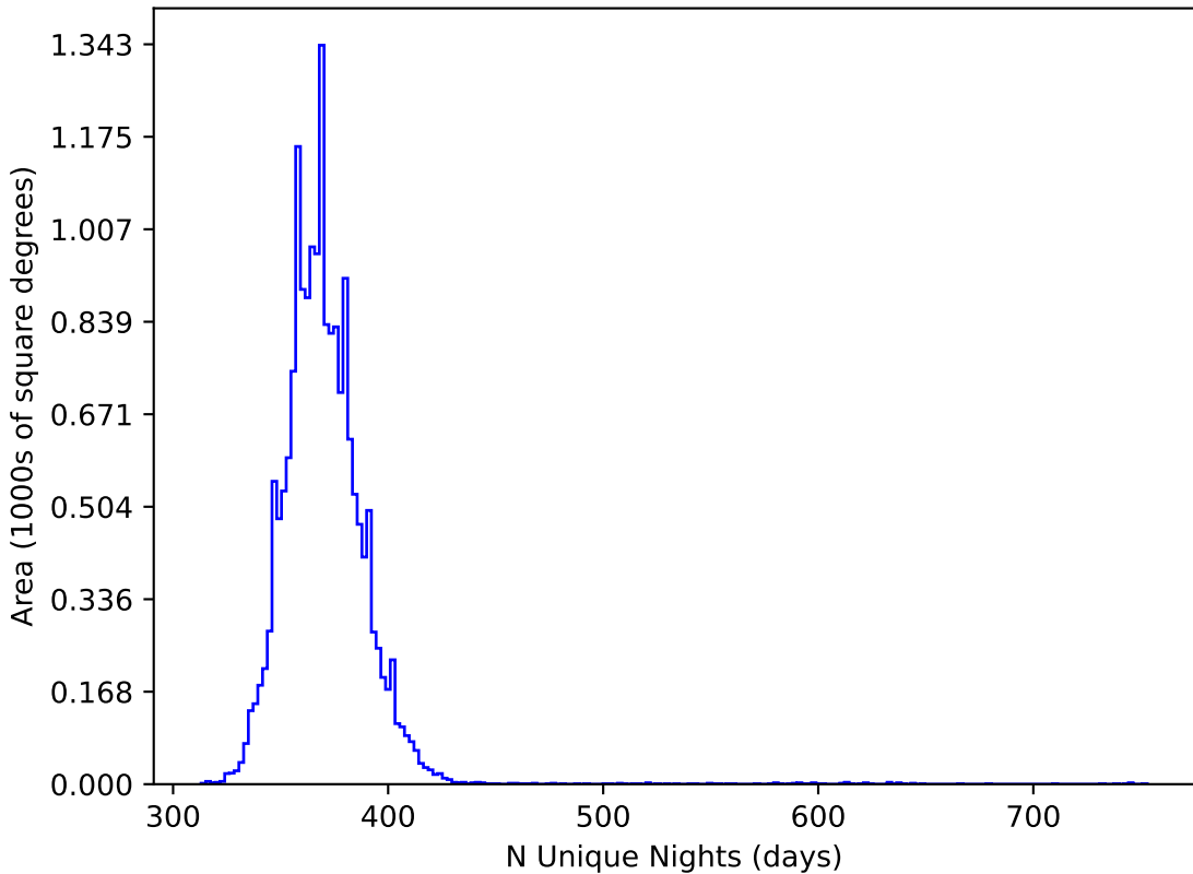
too_elab_r64_d2_giz_v3.4_10yrs WFD all bands: N Unique Nights
