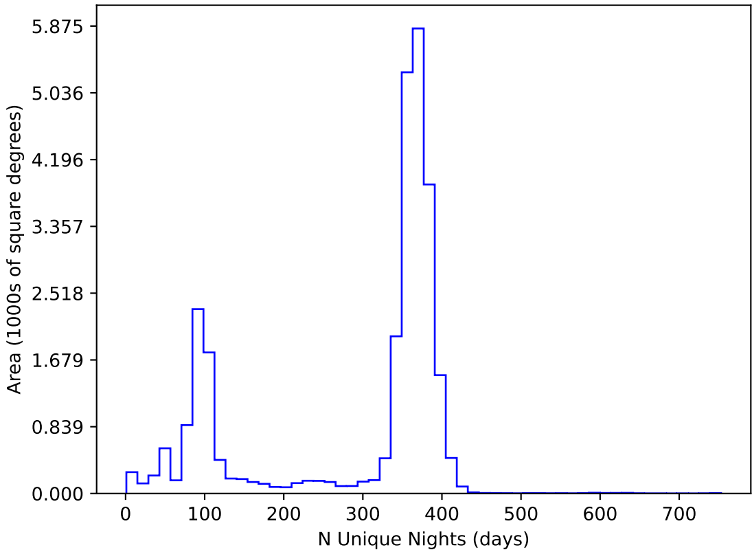
too_elab_r64_d2_giz_v3.4_10yrs All sky all bands: N Unique Nights
