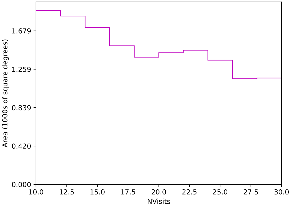
too_elab_r64_d2_giz_v3.4_10yrs Yr 3-4 z band: NVisits
