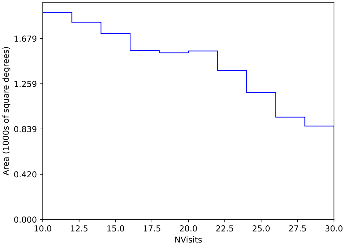
too_elab_r64_d2_giz_v3.4_10yrs Yr 3-4 y band: NVisits
