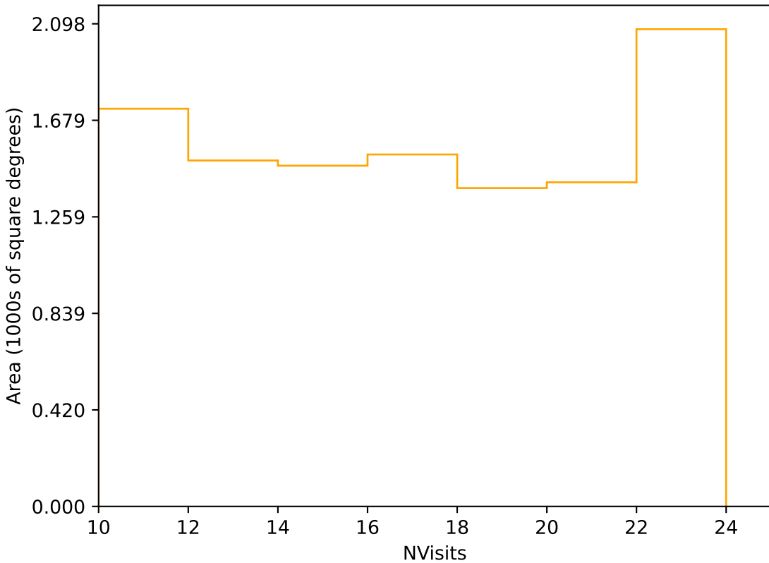
too_elab_r64_d2_giz_v3.4_10yrs Yr 3-4 r band: NVisits
