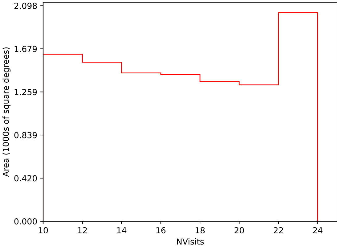
too_elab_r64_d2_giz_v3.4_10yrs Yr 3-4 i band: NVisits
