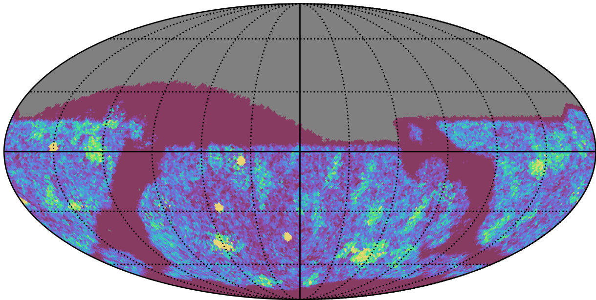
too_elab_r64_d2_giz_v3.4_10yrs Yr 1 z band: NVisits
