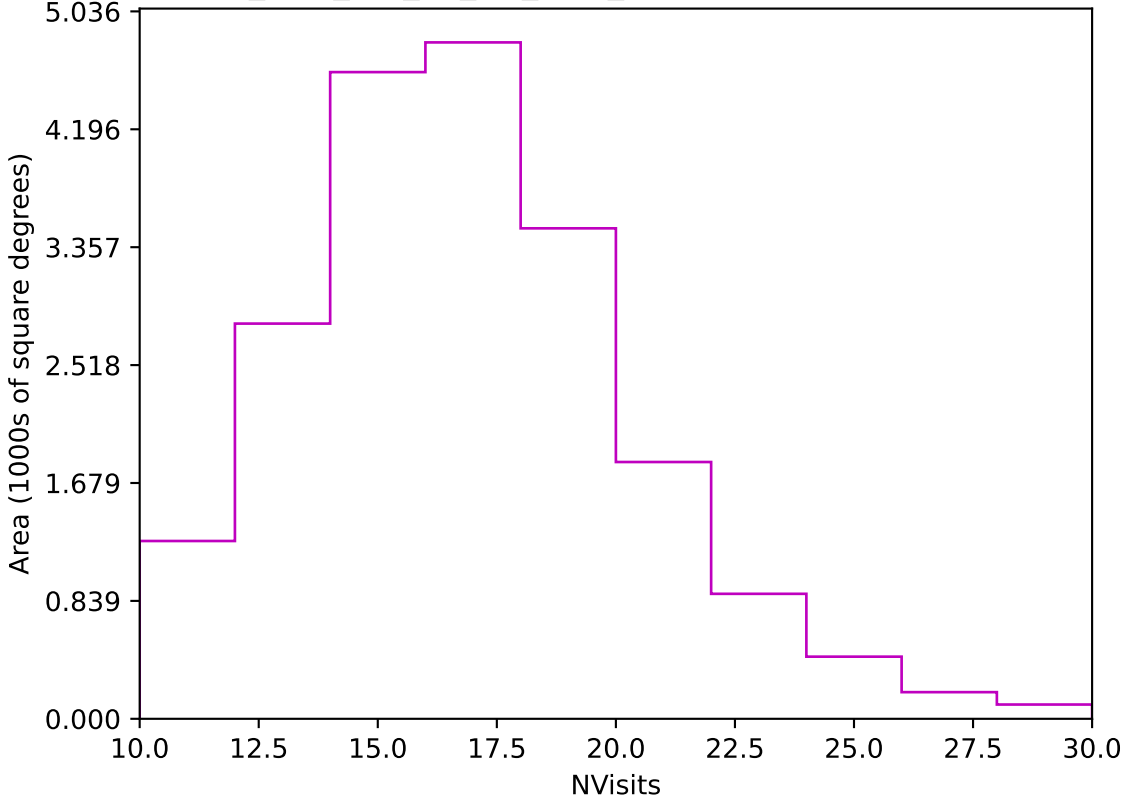
too_elab_r64_d2_giz_v3.4_10yrs Yr 1 z band: NVisits
