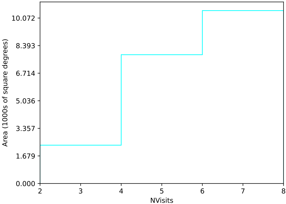
too_elab_r64_d2_giz_v3.4_10yrs Yr 1 u band: NVisits
