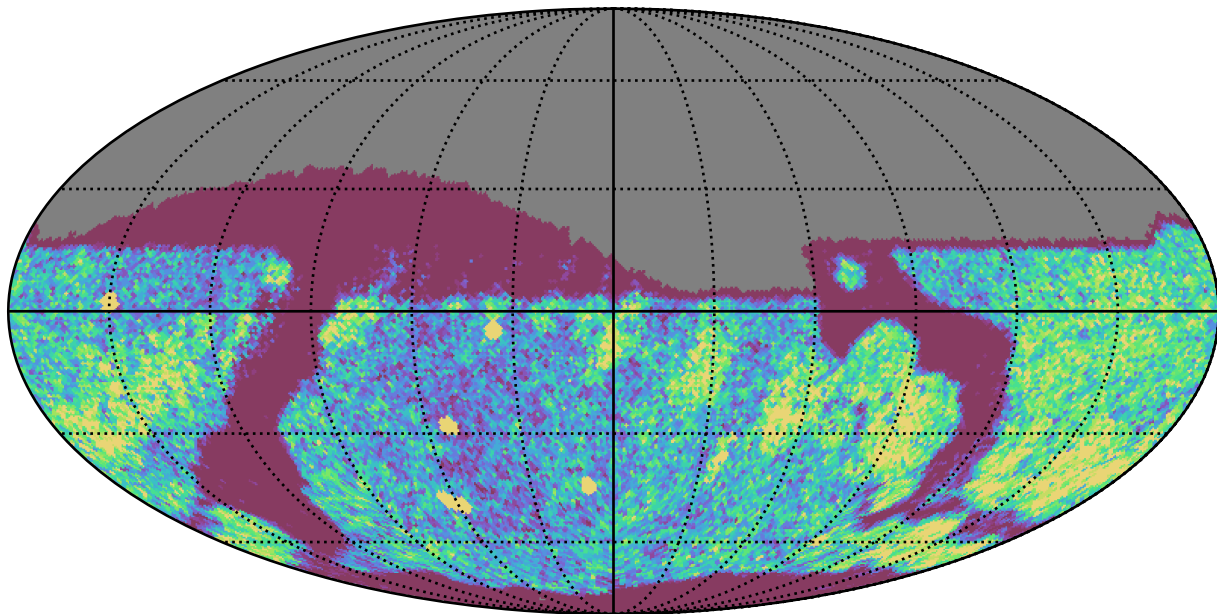
too_elab_r64_d2_giz_v3.4_10yrs Yr 1 r band: NVisits
