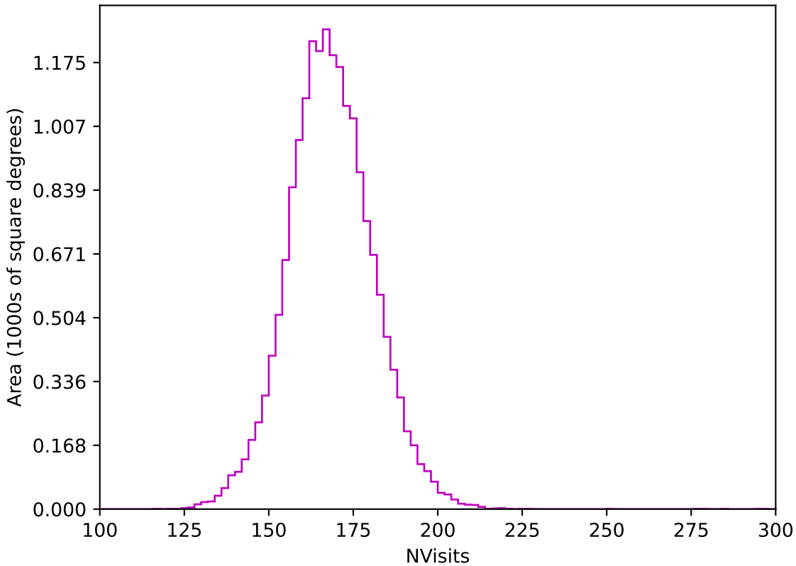
too_elab_r64_d2_giz_v3.4_10yrs WFD z band: NVisits
