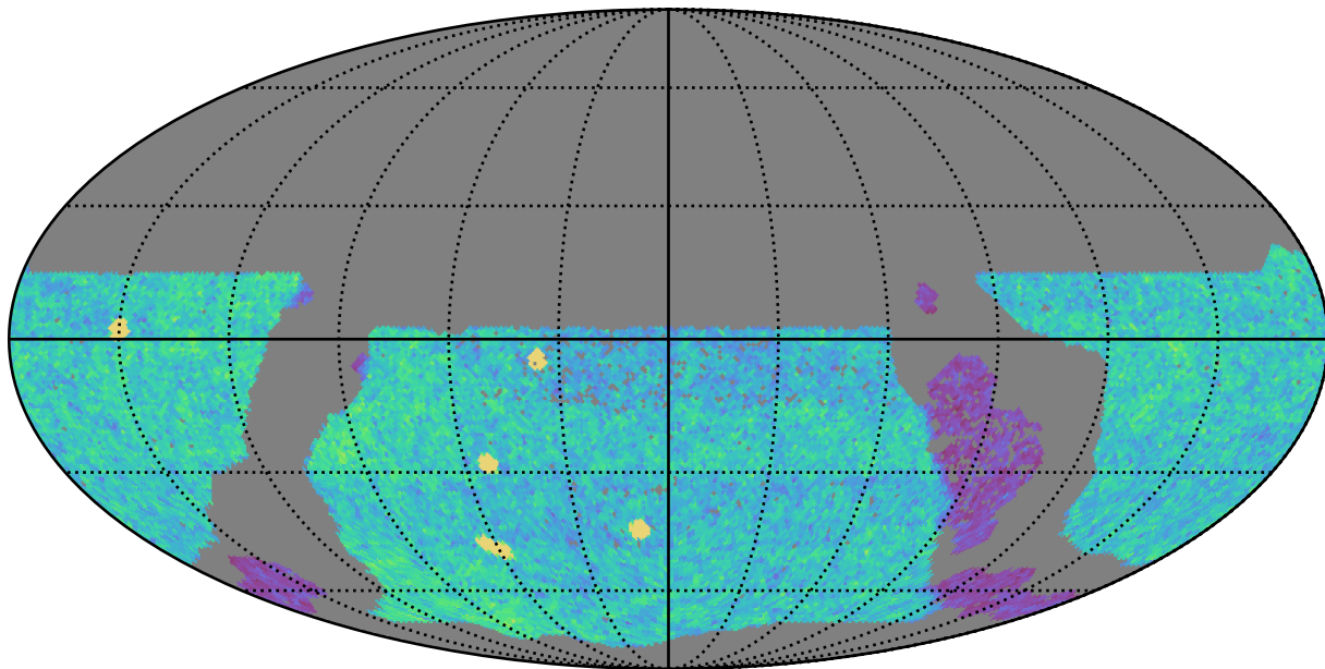
too_elab_r64_d2_giz_v3.4_10yrs WFD u band: NVisits
