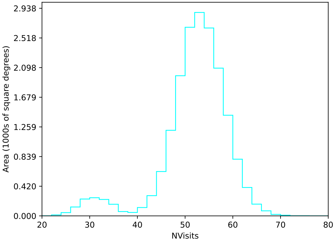
too_elab_r64_d2_giz_v3.4_10yrs WFD u band: NVisits
