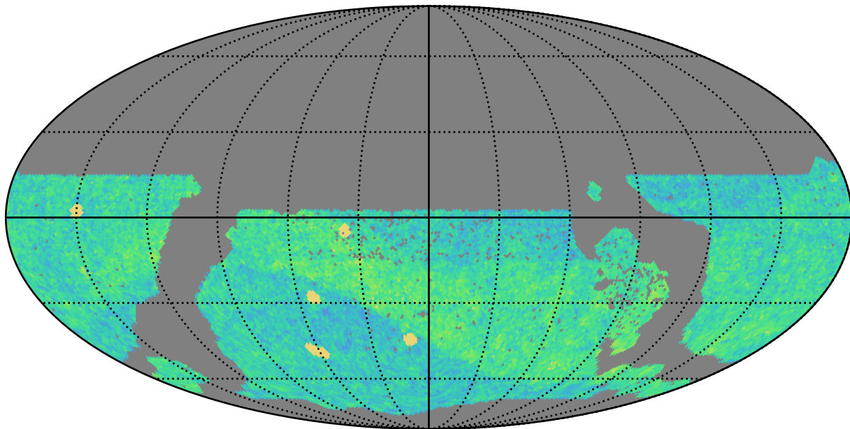
too_elab_r64_d2_giz_v3.4_10yrs WFD i band: NVisits
