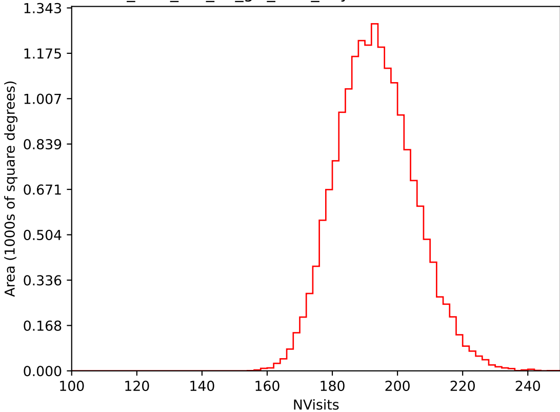
too_elab_r64_d2_giz_v3.4_10yrs WFD i band: NVisits
