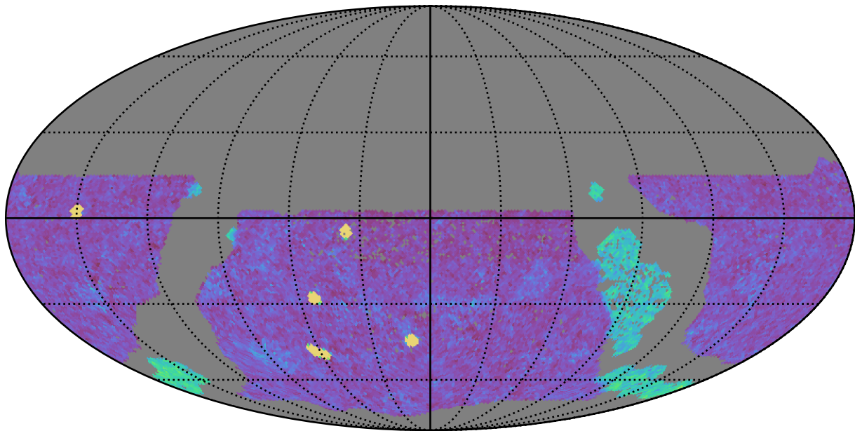
too_elab_r64_d2_giz_v3.4_10yrs WFD g band: NVisits
