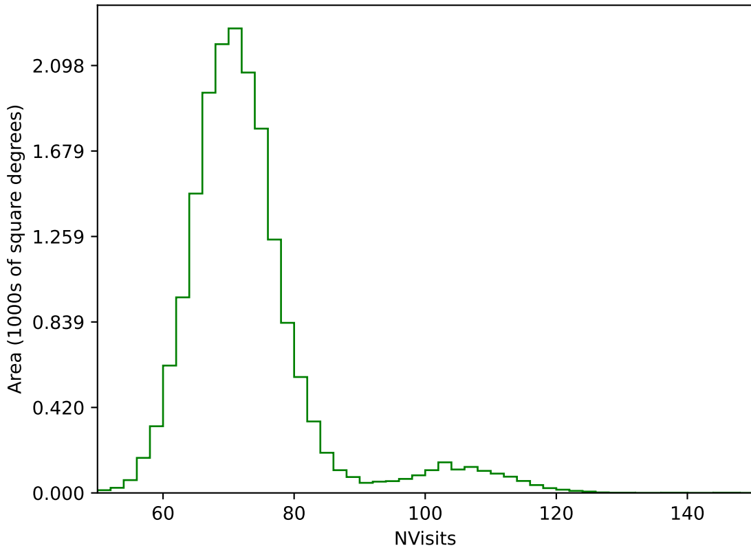
too_elab_r64_d2_giz_v3.4_10yrs WFD g band: NVisits
