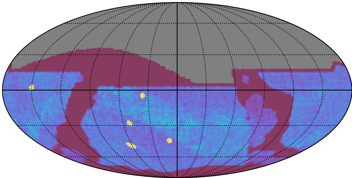
too_elab_r64_d2_giz_v3.4_10yrs All sky z band: NVisits
