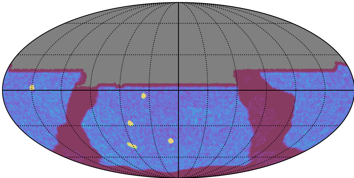
too_elab_r64_d2_giz_v3.4_10yrs All sky y band: NVisits
