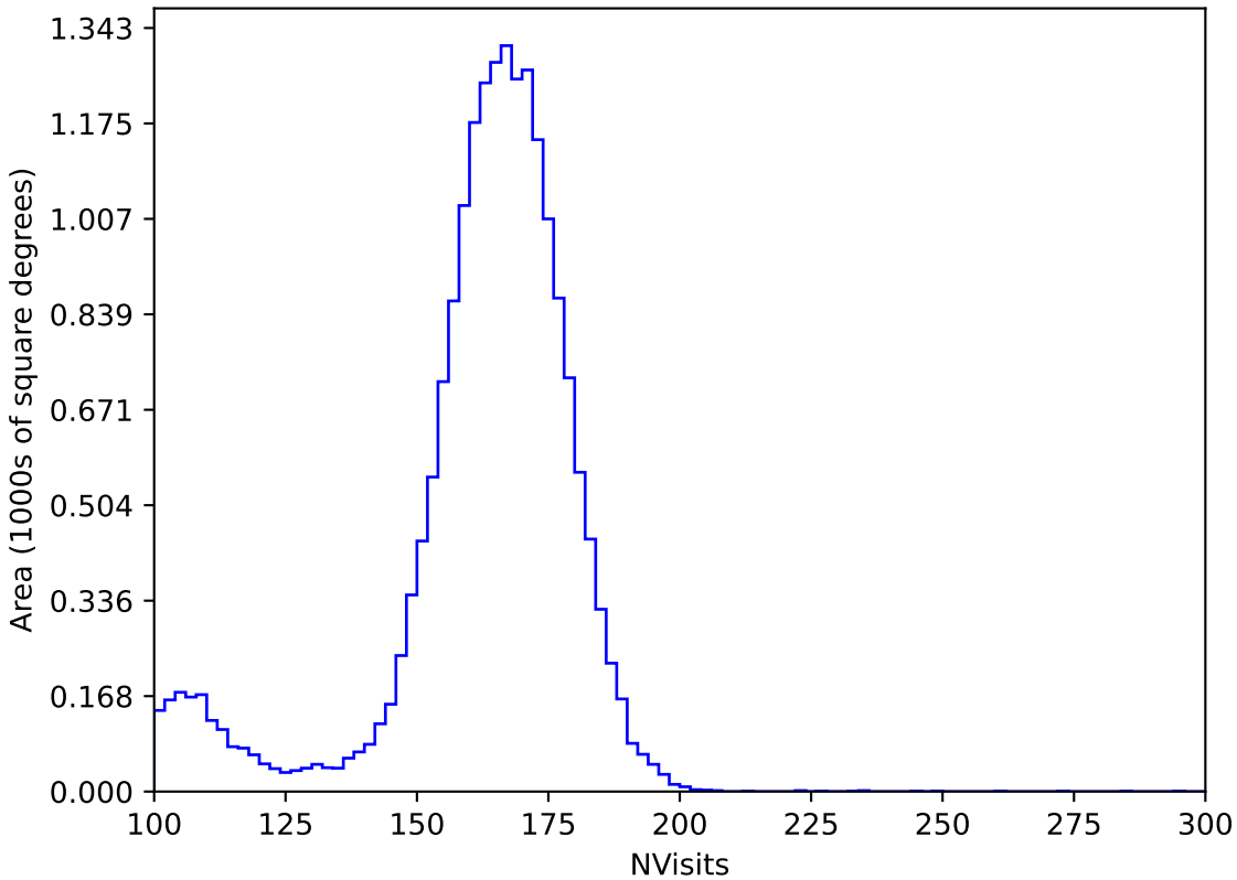
too_elab_r64_d2_giz_v3.4_10yrs All sky y band: NVisits
