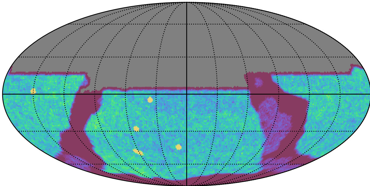
too_elab_r64_d2_giz_v3.4_10yrs All sky u band: NVisits
