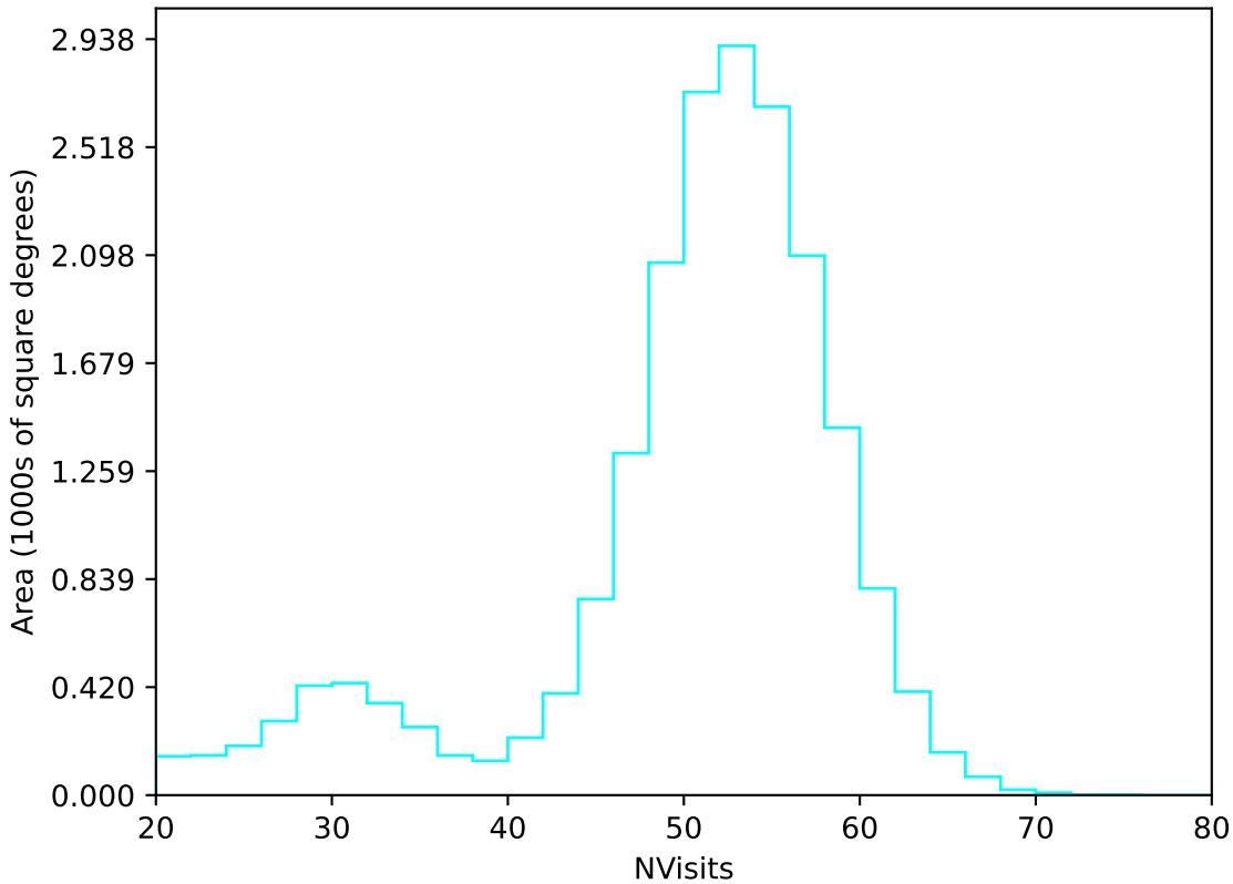
too_elab_r64_d2_giz_v3.4_10yrs All sky u band: NVisits
