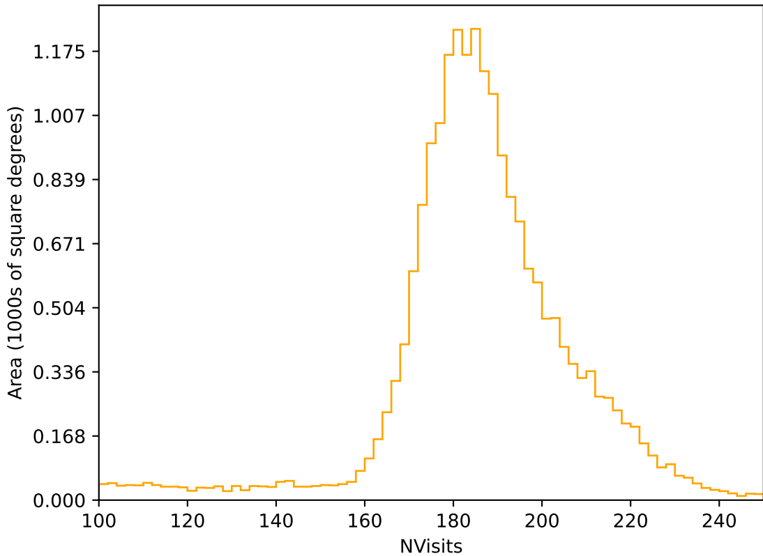
too_elab_r64_d2_giz_v3.4_10yrs All sky r band: NVisits
