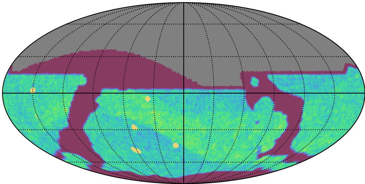
too_elab_r64_d2_giz_v3.4_10yrs All sky i band: NVisits
