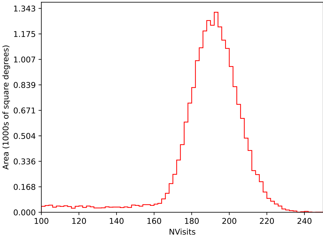
too_elab_r64_d2_giz_v3.4_10yrs All sky i band: NVisits
