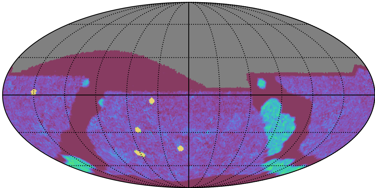
too_elab_r64_d2_giz_v3.4_10yrs All sky g band: NVisits
