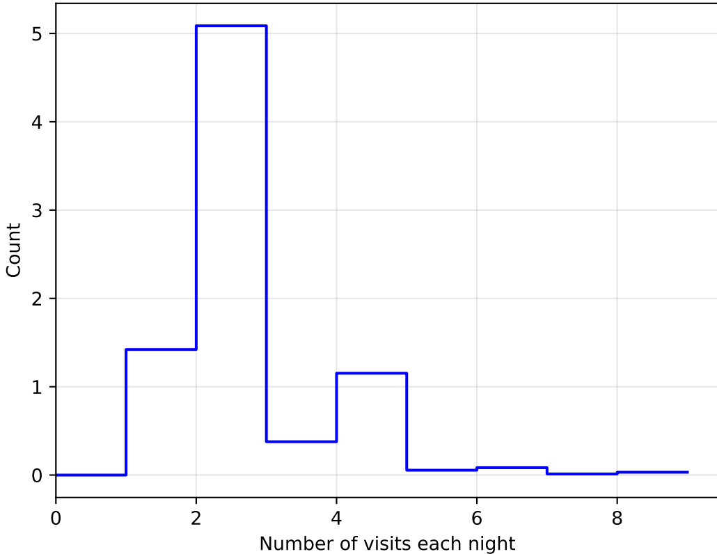
too_elab_r64_d2_giz_v3.4_10yrs WFD: NVisitsPerNight
