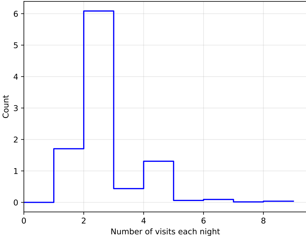
too_elab_r64_d2_giz_v3.4_10yrs All sky: NVisitsPerNight
