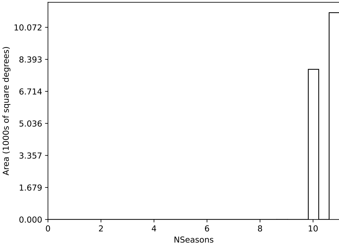
too_elab_r64_d2_giz_v3.4_10yrs WFD all bands: NSeasons
