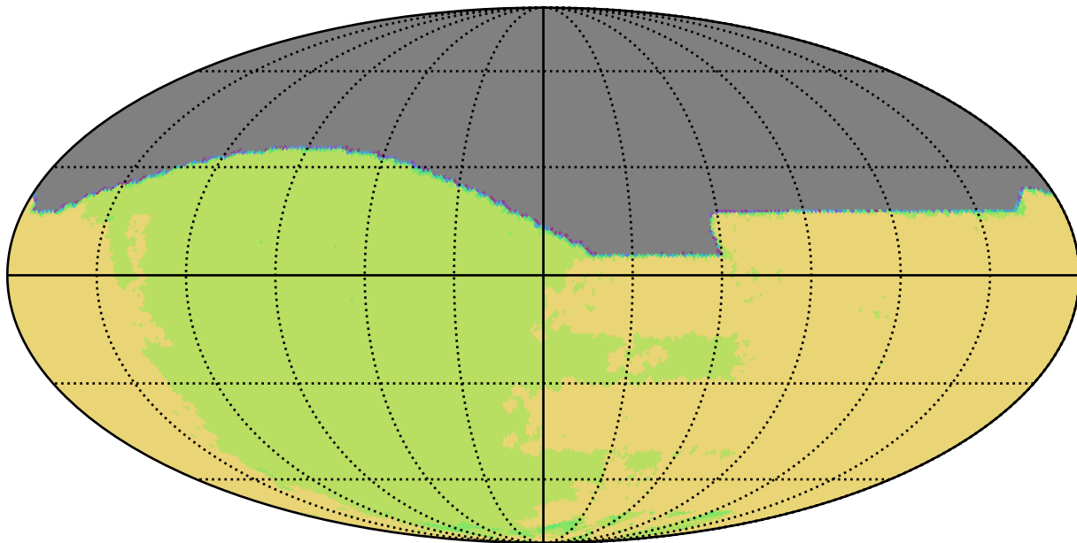
too_elab_r64_d2_giz_v3.4_10yrs All sky all bands: NSeasons
