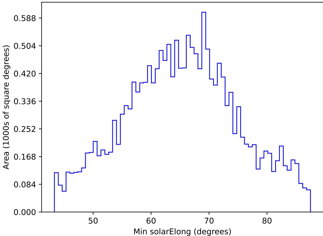
too_elab_r64_d2_giz_v3.4_10yrs WFD y band: Min solarElong
