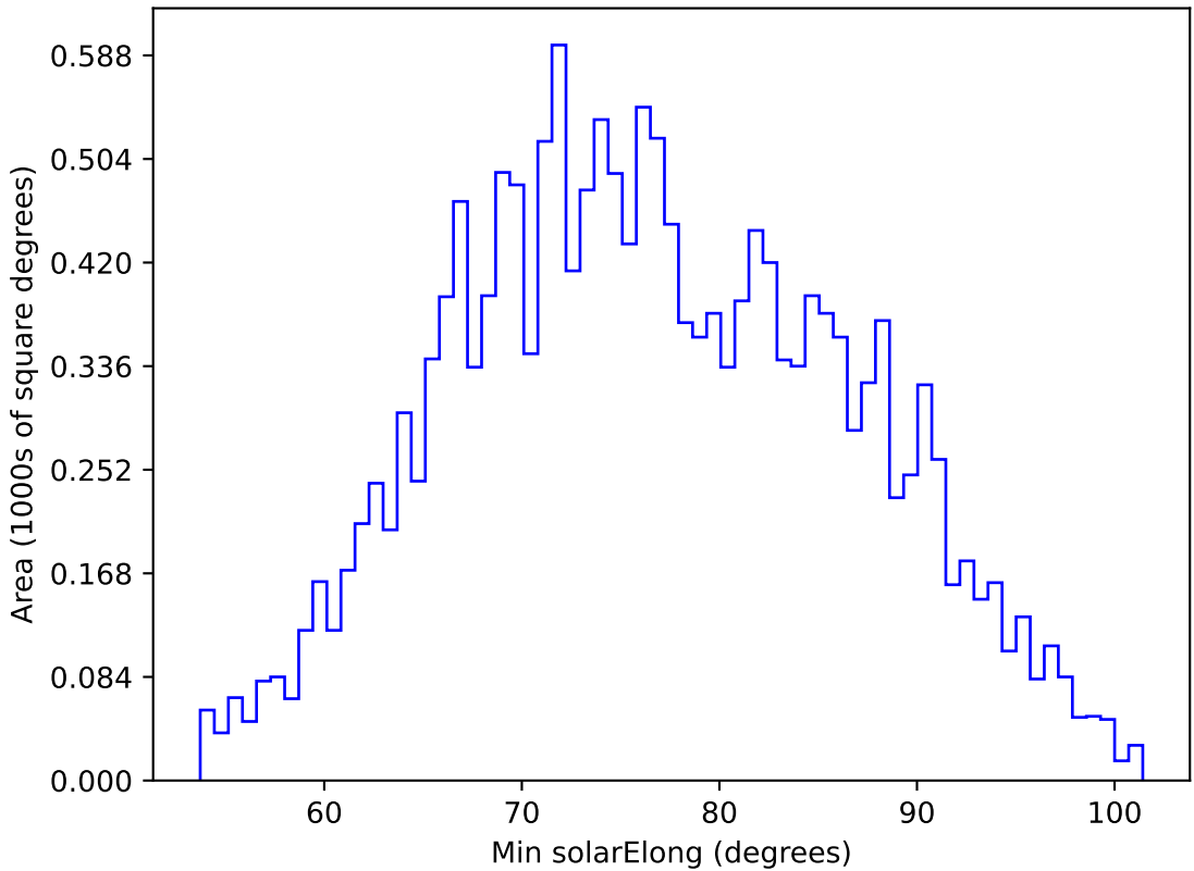
too_elab_r64_d2_giz_v3.4_10yrs WFD u band: Min solarElong
