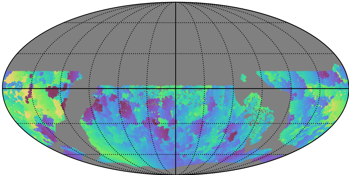
too_elab_r64_d2_giz_v3.4_10yrs WFD g band: Min solarElong
