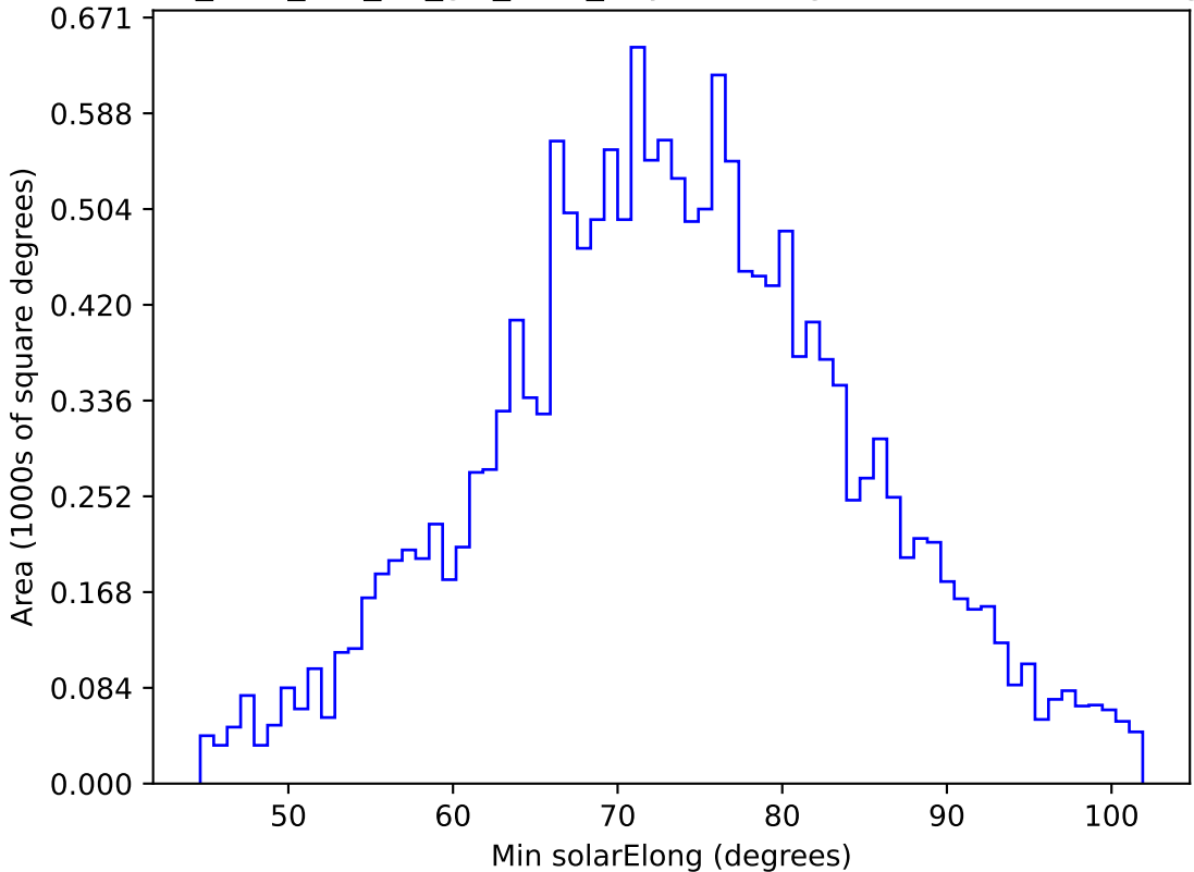
too_elab_r64_d2_giz_v3.4_10yrs WFD g band: Min solarElong
